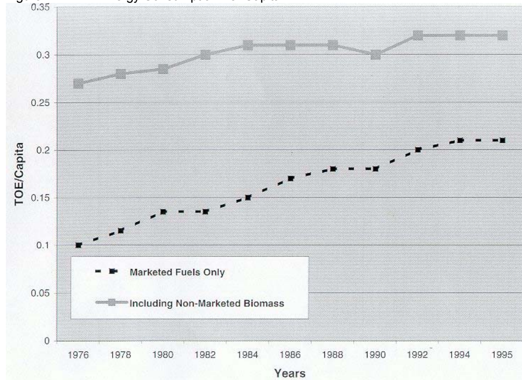
Figure 2: Final Energy Consumption (Marketed Fuels Only)
